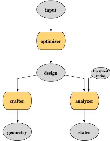
Figure 1. OpenProp information flow chart
